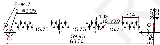
PCB Layout
